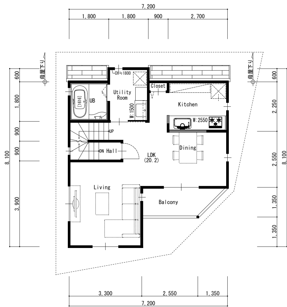
2 F PLAN
