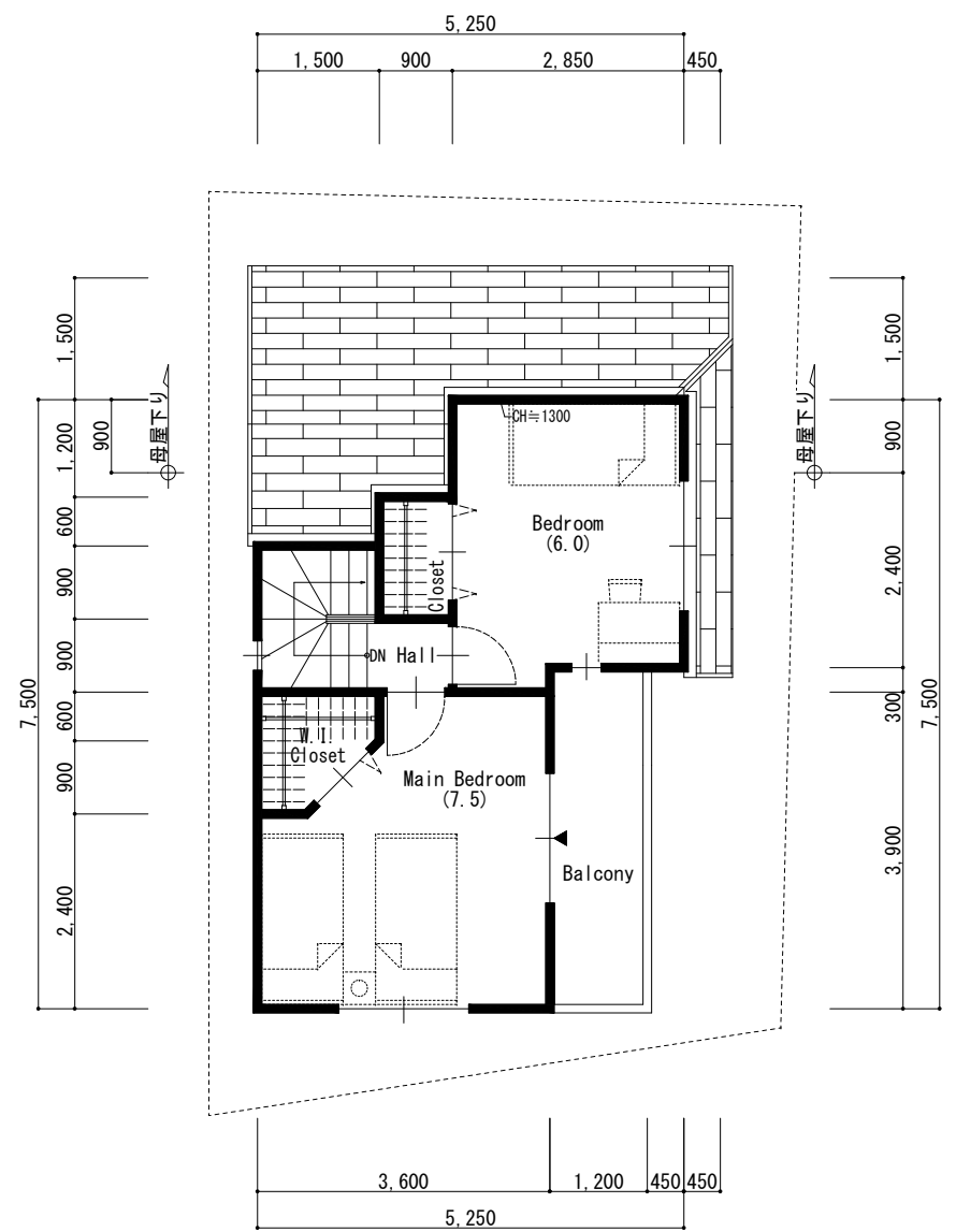
3 F PLAN
