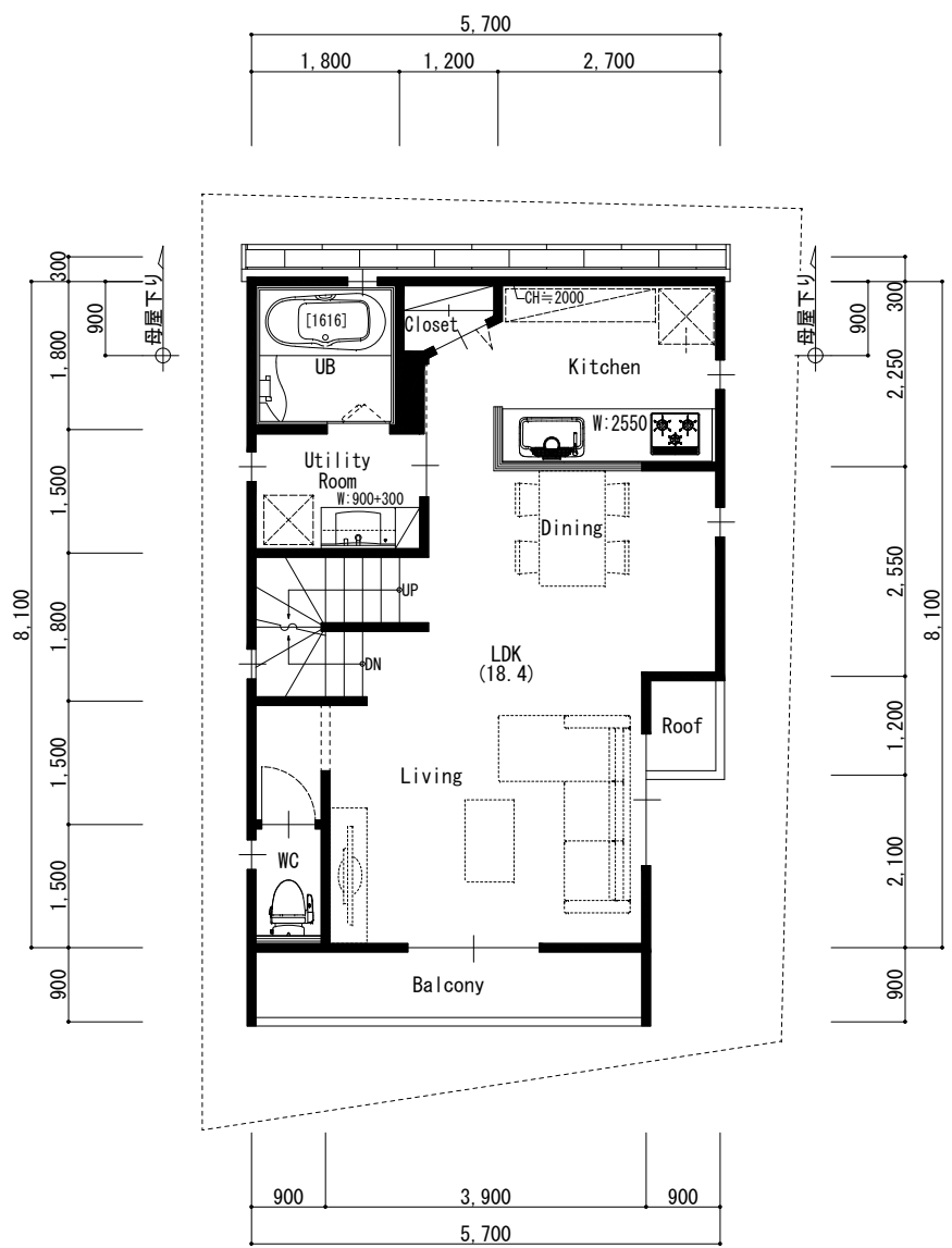
2 F PLAN
