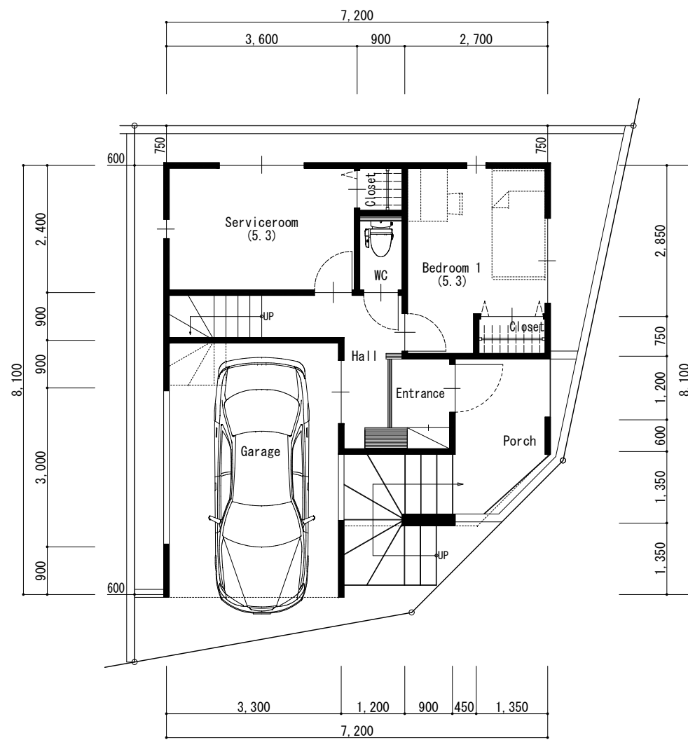
1 F PLAN
