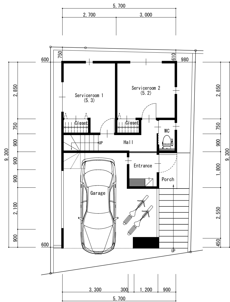
1 F PLAN
