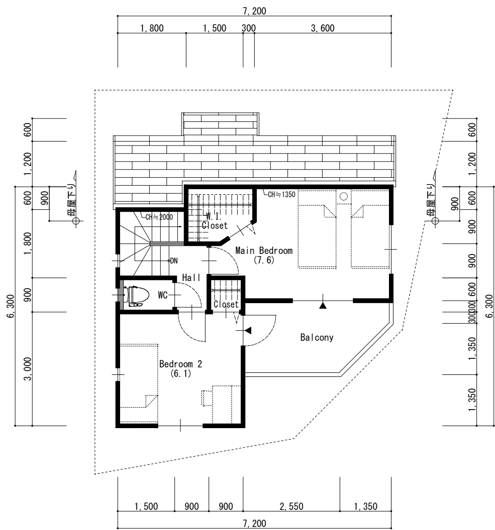
3 F PLAN
